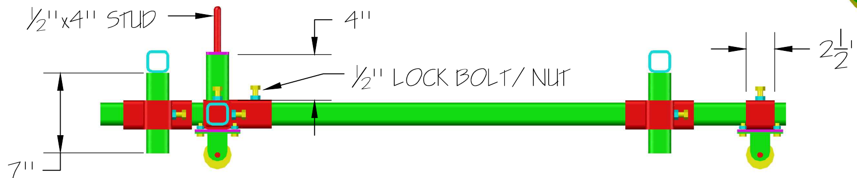
SIDE VIEW
